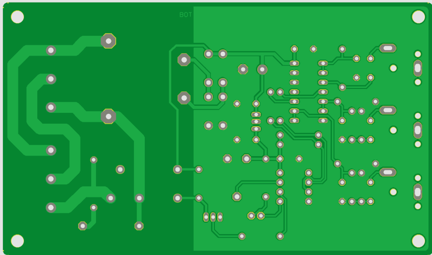
E750161 PCB view BOTTOM (bottomview)
